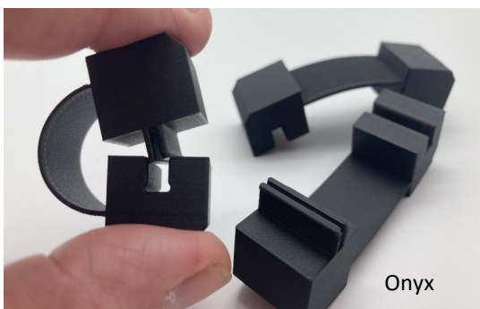
Build area 320 x 132 x 154mm
