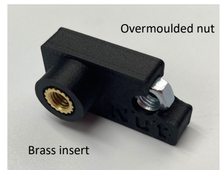
Twin Filament Build
