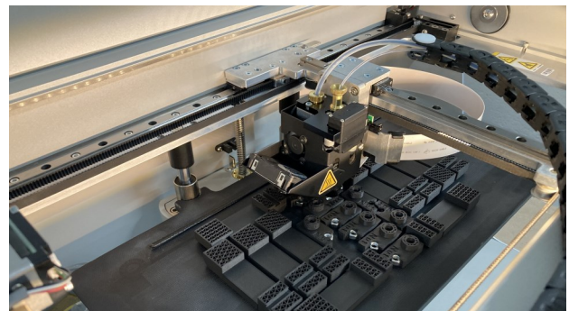
Twin Filament Build
